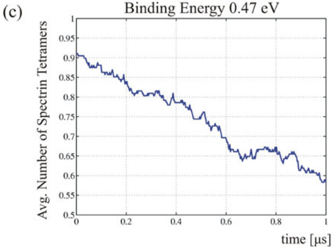
Fig. 7. Progressive decrease of the dimer - dimer association integrity during shearing (with no chemically inserted energy) at 0.6 eV ( a ), 0.56 eV ( b ), and 0.47 eV ( c ) dimer-dimer association energy.
