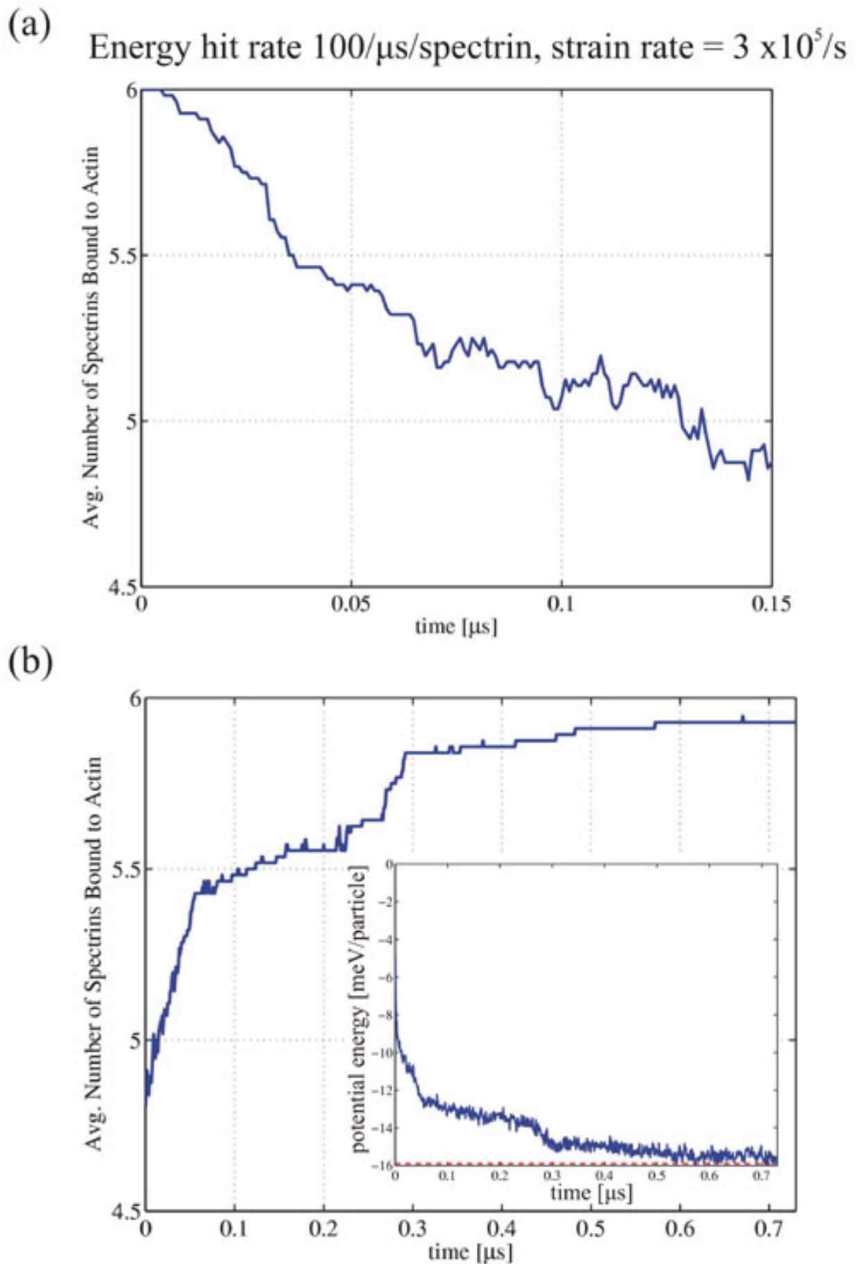
Fig. 6. (a) Kinetics of defect creation and accumulation at energy hit rate 100 per \mu\text{s} (very high). (b) Recovery
